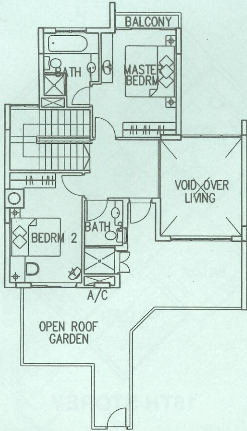
15TH STOREY
