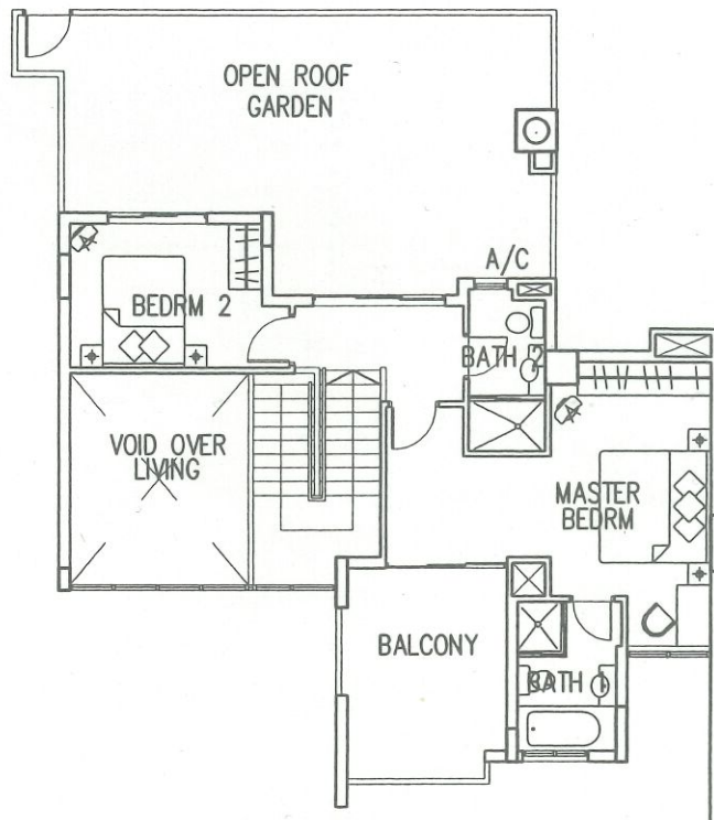
15TH STOREY
