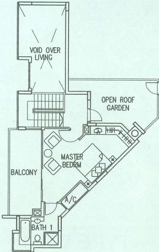
15TH STOREY
