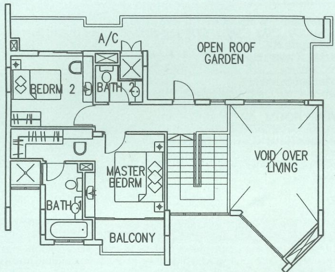
15TH STOREY
