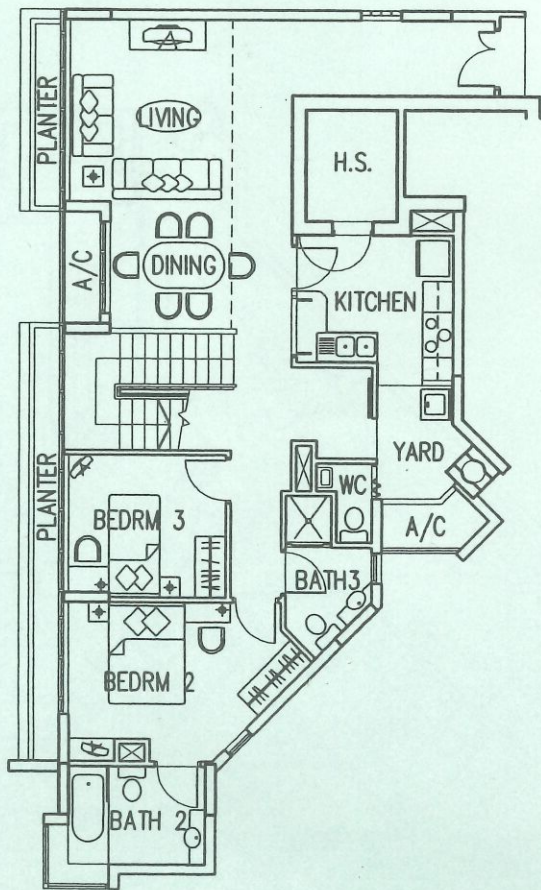
14TH STOREY
