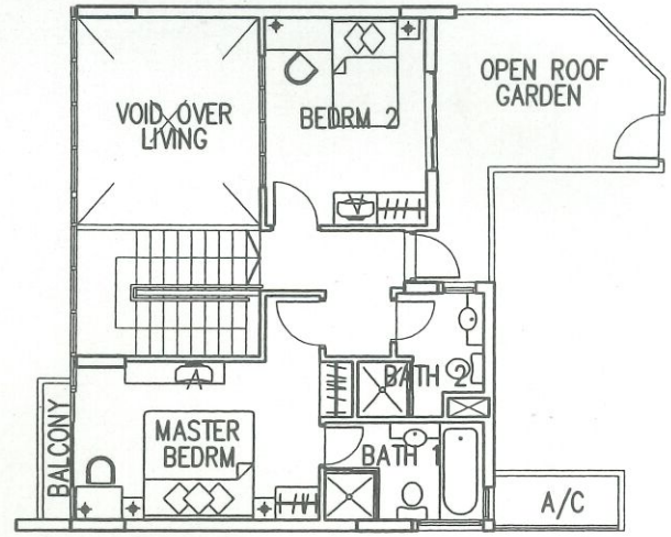
15TH STOREY
