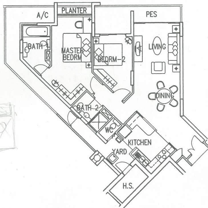
TYPE B2P1
